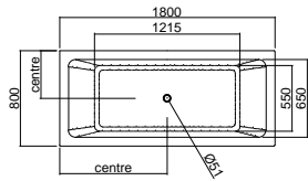
Height with optional upstand 500 mm
