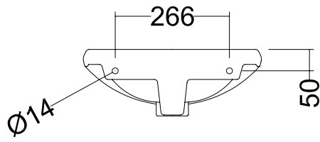
Rear Detail of Basin
